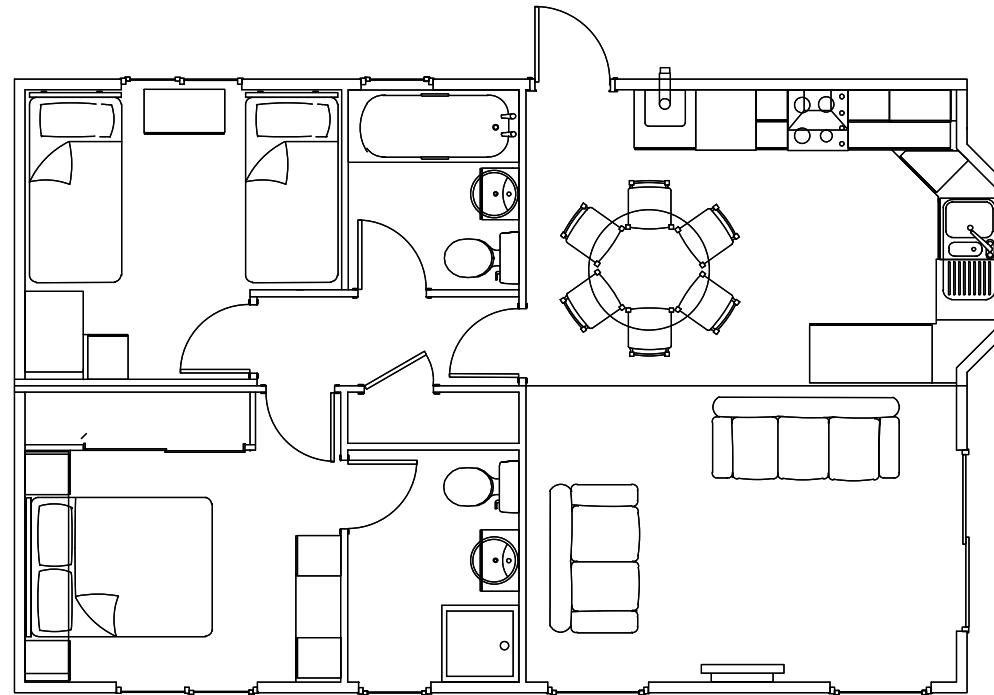
BLENHEIM 31' x 20' (2 BED)
