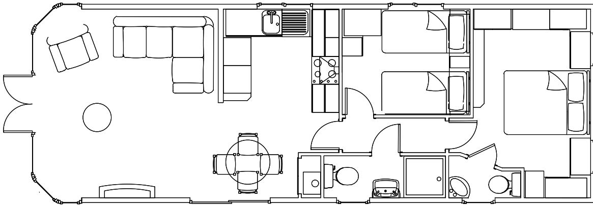
Seawood 40' x 12'
